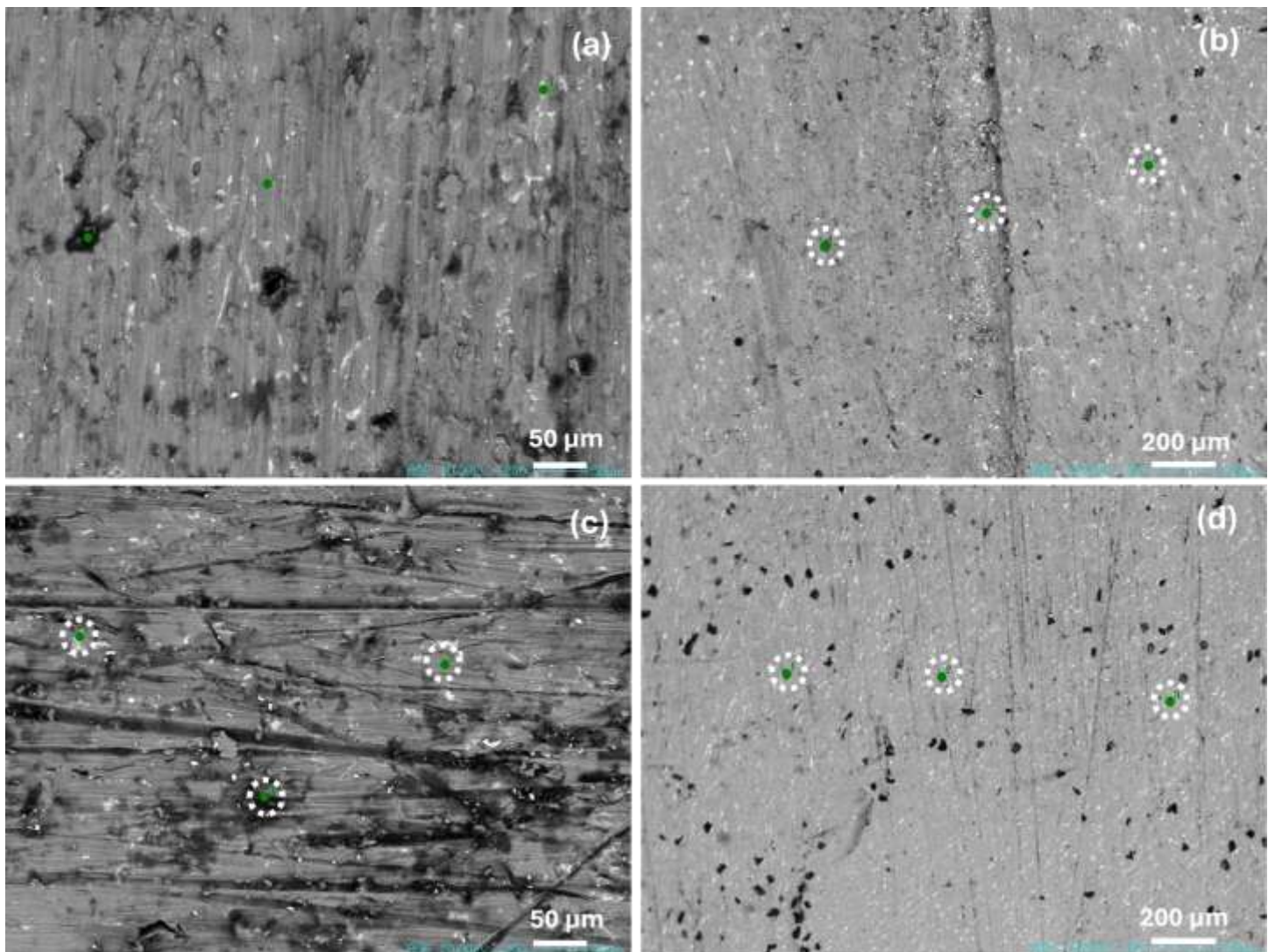
Fig. 4. SEM images of (a) Sample 0, (b) Sample 3, (c) Sample 6, (d) Sample 9. The dotted white circles indicating the presence of TiO 2 particles.
